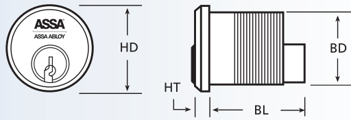
Mortise Cylinder Key: HD – Head Diameter
